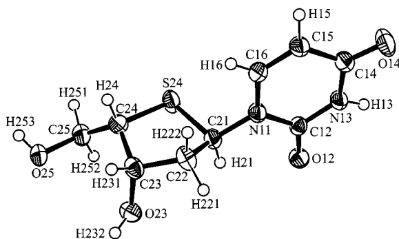
Figure 1. ORTEP view of the X-ray diffraction structure of uridine derivative \alpha - 23 ; thermal ellipsoids are drawn at the 50% probability level
