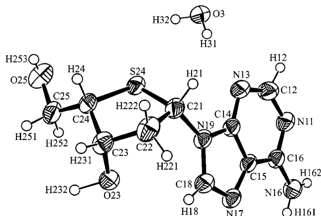
Figure 3. ORTEP view of the X-ray diffraction structure of adenosine derivative \beta -36 with one molecule of crystal water; thermal ellipsoids are drawn at the 50% probability level
