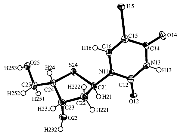
Figure 2. ORTEP view of the X-ray diffraction structure of 5-iodouridine derivative \alpha - 28 ; thermal ellipsoids are drawn at the 50% probability level
